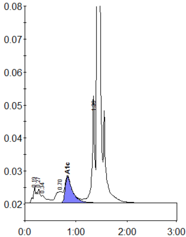
Peak table - ID: 10676965
